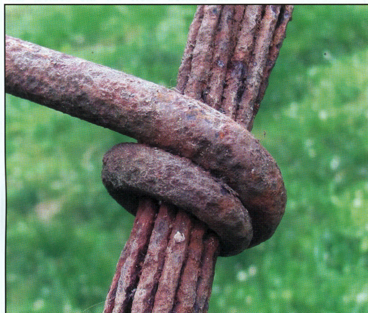
This iron suspender tightly surrounds the 18-wire cable bundle. Note the tapered end of the suspender iron as it snakes around the cable.
